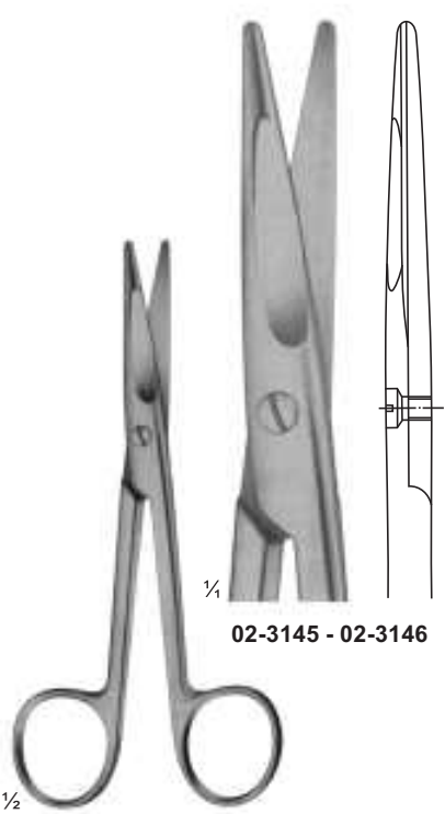
1/2 02-3145 - 02-3146 MAYO-STILLE With chamfered blades 02-3145 (140 mm) 02-3146 (170 mm)
